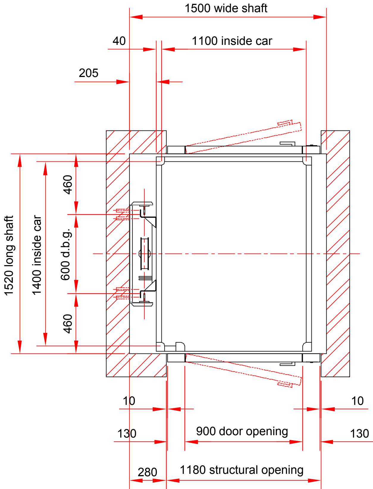
Drawing Title : XL 1100 x 1400 OPEN THROUGH IN BRICK SHAFT
