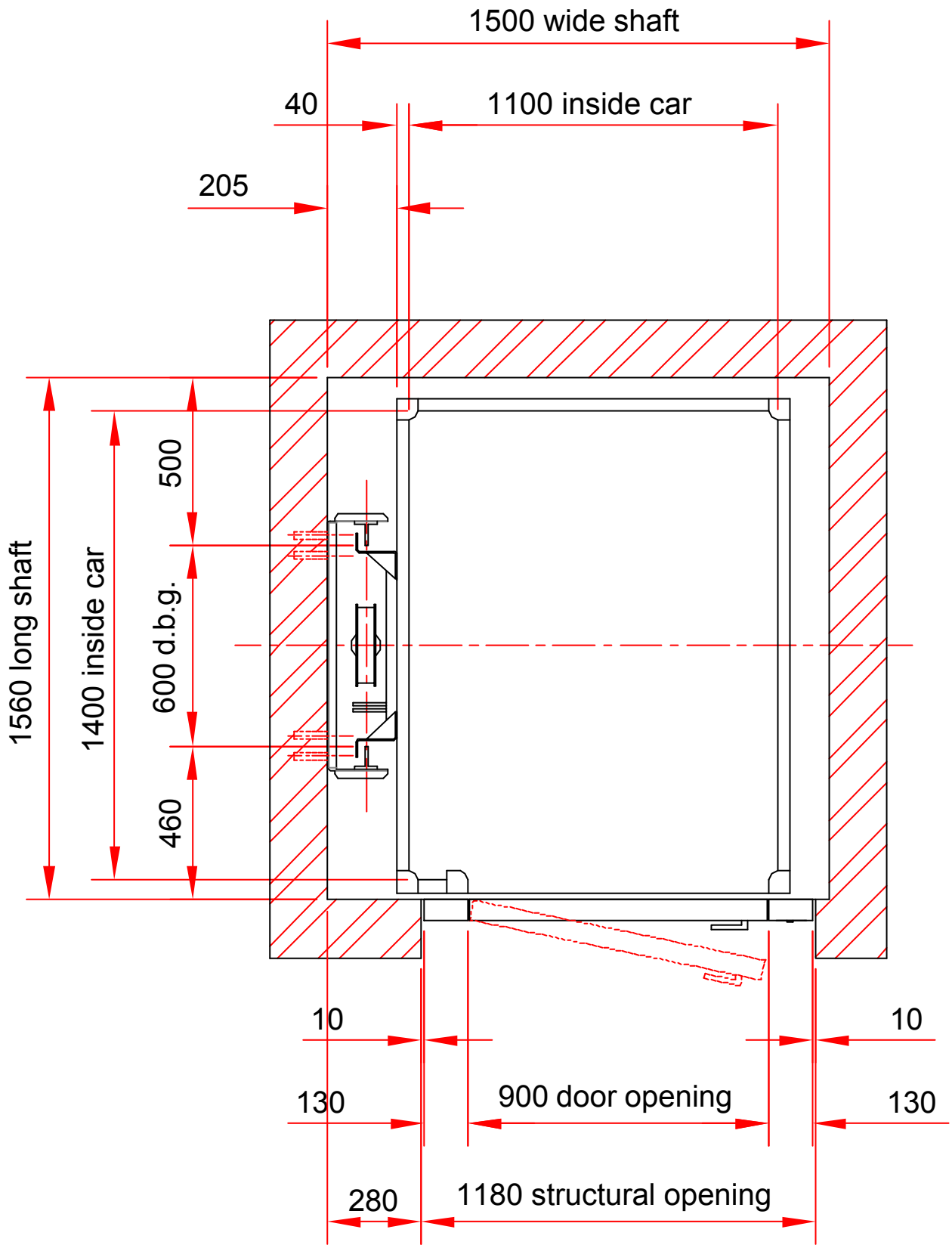
Drawing Title : XL 1100 x 1400 OPEN FRONT ONLY IN BRICK SHAFT
